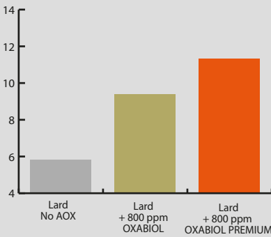
Rancimat Test at 120°C - Lard
